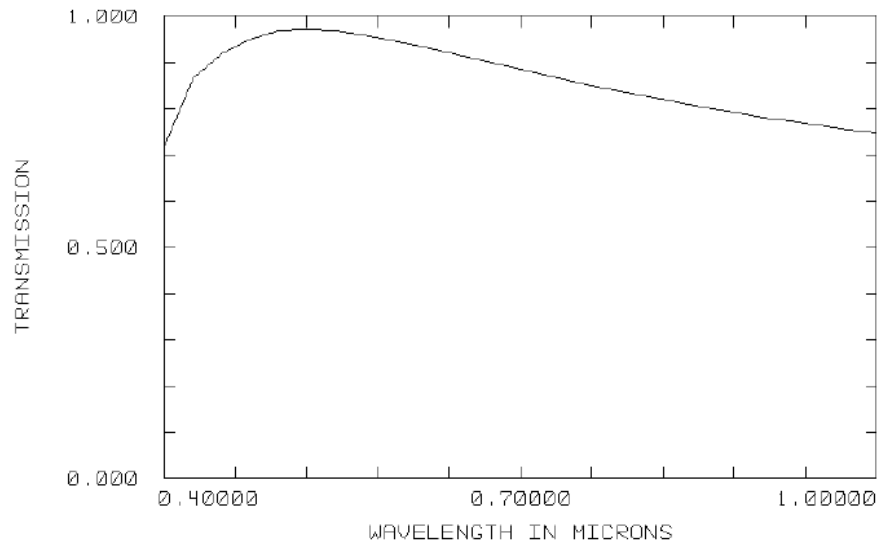
LM35JCM Transmission
