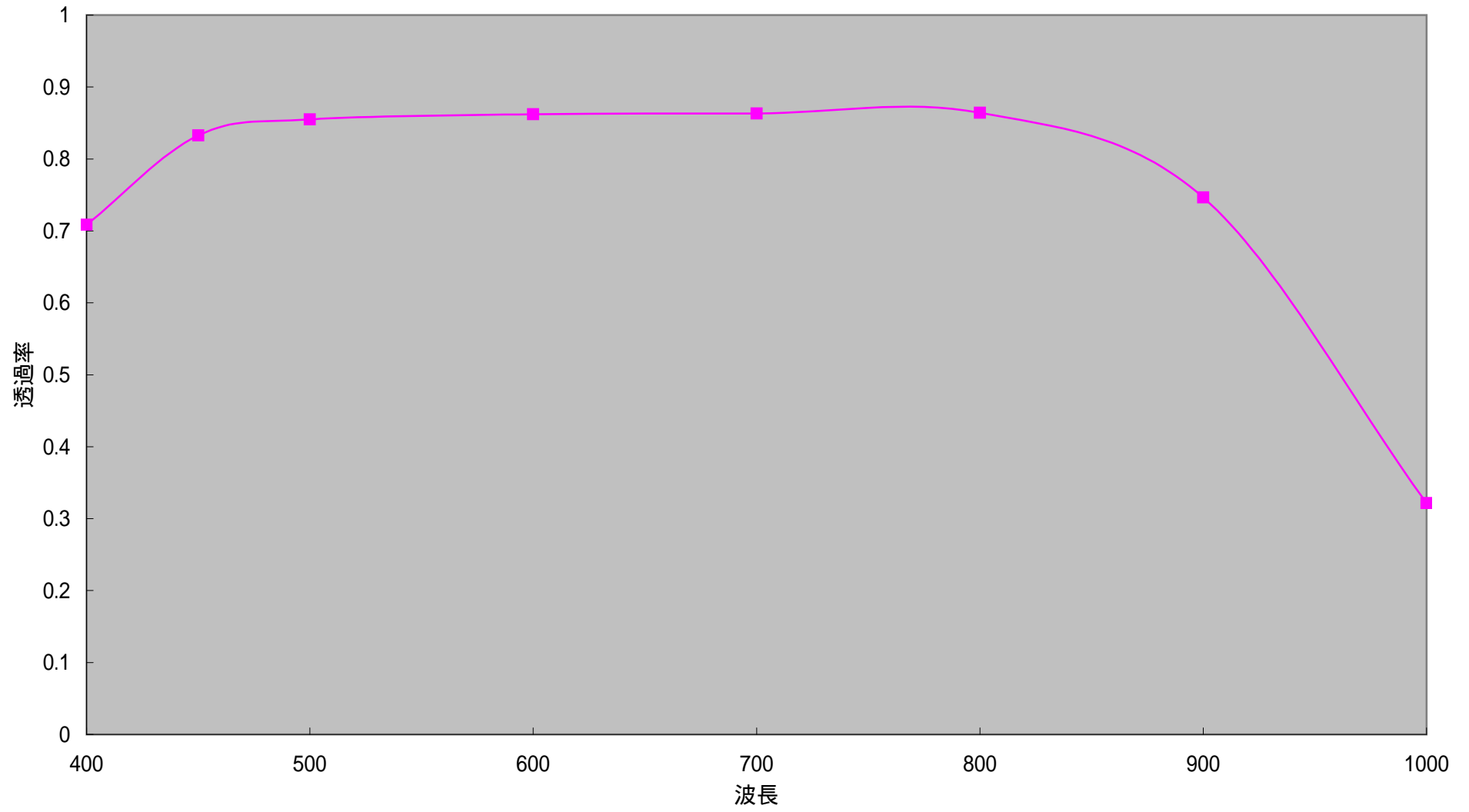
LM25JC10M 透過率
