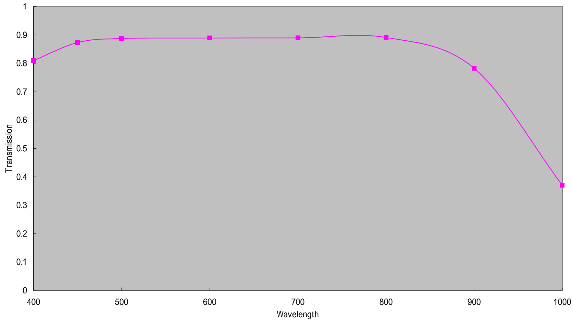
LM5JC10M Transmission
