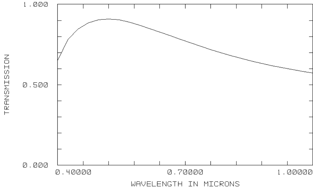
TRANSMISSION VS. WAVELENGTH
